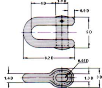
k. Swivel Shackle (All Grades)
