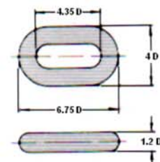
c. End Link
