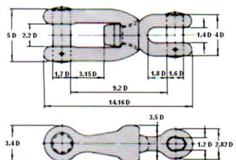
k. Swivel Shackle (All Grades)
