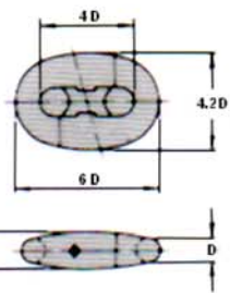
h. Pear End Shackle
