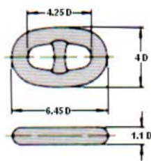
b. Englarged Link
