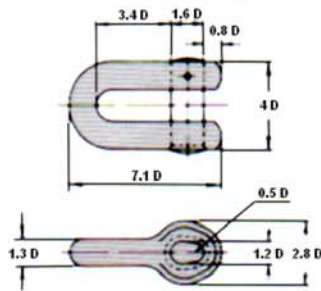
j. Swivel (Grade 2)
