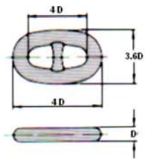
a. Common Link
