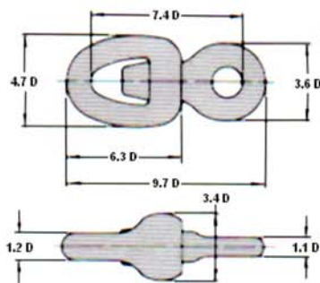
j. Swivel (Grade 2)
